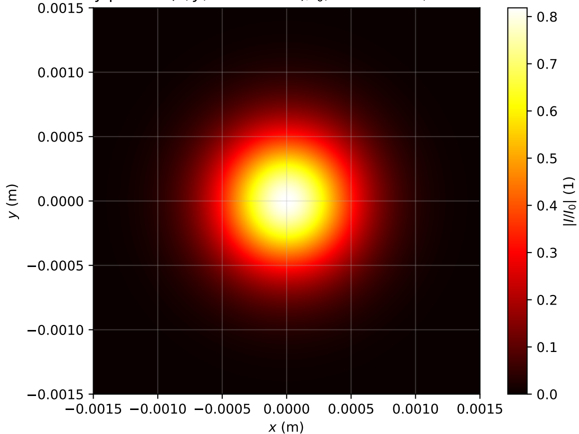
Intensity profile I(x, y, z = 1.433m)/I_0 , Pin=0.3Pcr, artificial time
